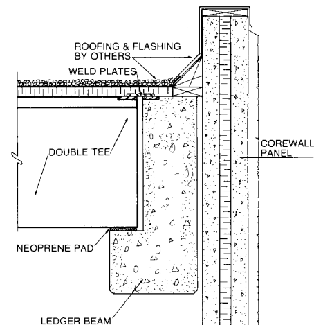
DOUBLE TEE BEARING ON LEDGER BEAM
