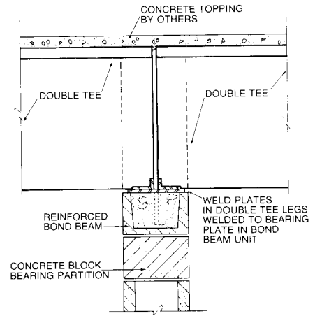
DOUBLE TEES BEARING ON MASONRY WALL
