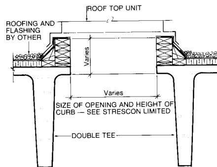
DOUBLE TEE WITH FRAMED OPENING
